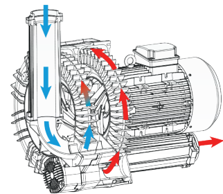
Series: TD Twin impeller Double stage
