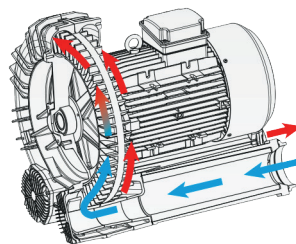
Series: MD Single impeller Double stage
