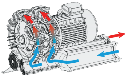
Series: TS Twin impeller Single stage
